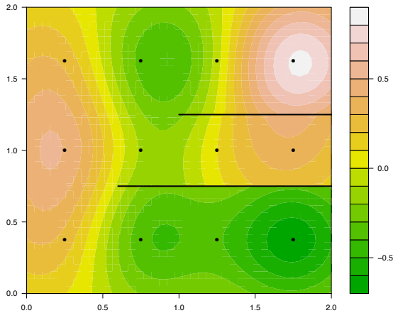
Figure 1: Toy example of the emulator adjusted expectation for a function with a 2-dimensional input space. The black lines depict the discontinuities and the black points the model run locations.
